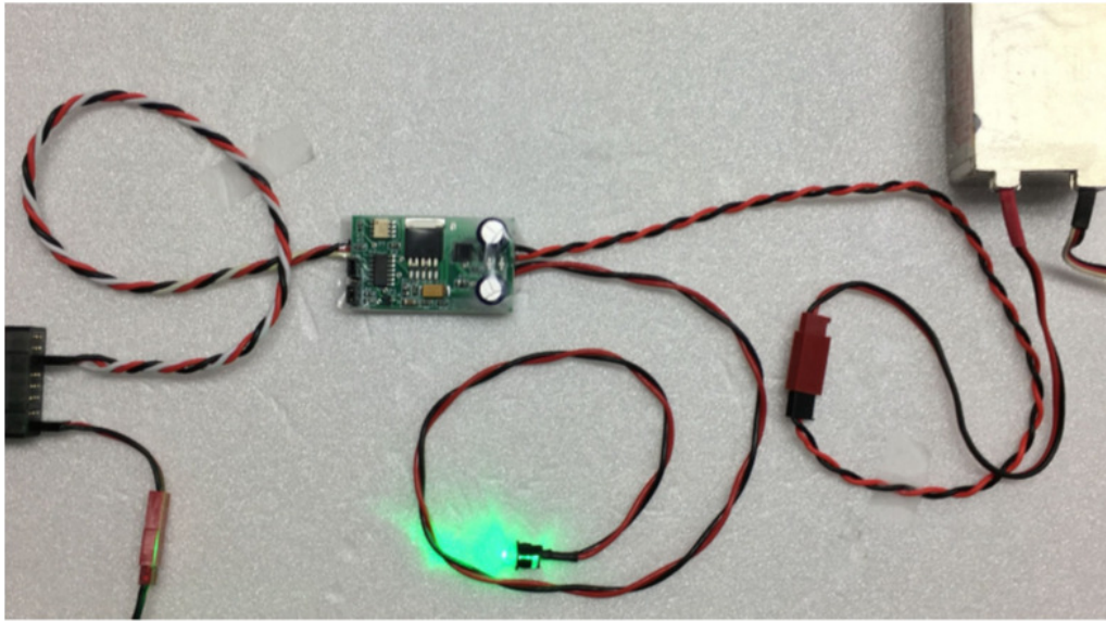
Figure 2 – Ultra IBEC HV Connection to Receiver and CDI Module
